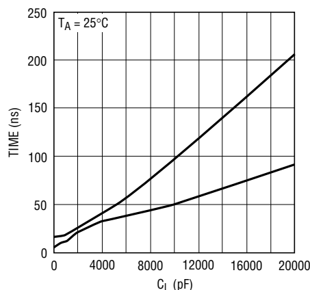
G1 Rise and Fall Time vs C_L
